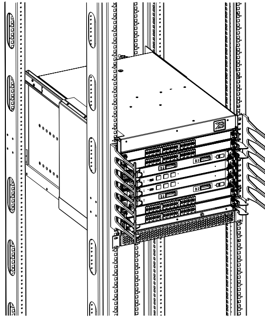
FIGURE 1 Vertical cable management finger assemblies
